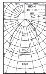
Candlepower Curve
