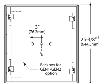
Top View (Flange Version)
