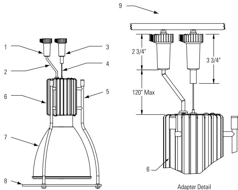
Typical complete installation shown (Power Head, Reflector and Aperture Disk must be ordered separately).
