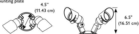
double CEF with round mounting plate
