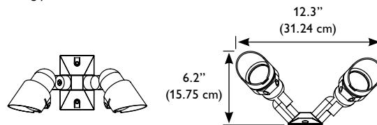
double CEF with rectangular mounting plate
