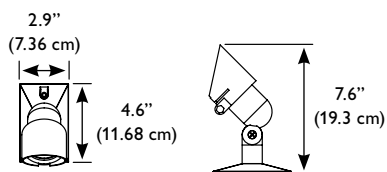
single CEF with rectangular mounting plate
