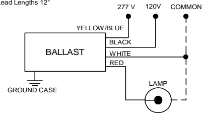
F-Can Wiring Diagram
