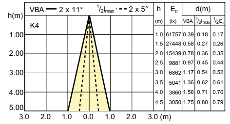
LDBE_CDMR111E_0007-Beam diagram
