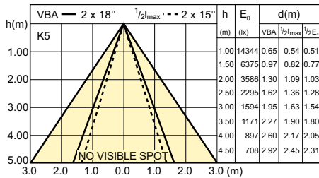
LDBE_CDM-R-E_0013-Beam diagram
