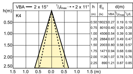
LDBE_CDM-Rm_20W_25D_0003-Beam diagram
