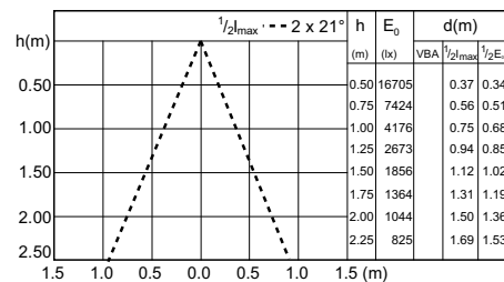
LDBE_CDM-Rm_35W_930_40D-Beam diagram
