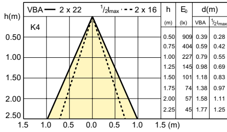
LDBE_HALUPAB_20W_32D-Beam diagram
