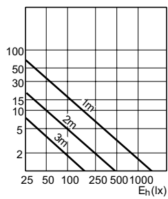
LDAC_HPAR30S_75W_30D-Accent diagram
