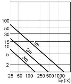
Accent Diagram - HalogenA Par30s 75W E27 230V 25D 1CT/15
