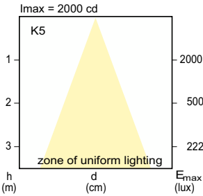
Beam diagram - HalogenA Par30s 75W E27 230V 25D 1CT/15
