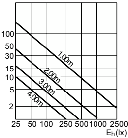
Accent Diagram - Alu111 50W 4000h G53 12V 24D 1CT/6
