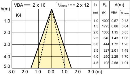
Beam diagram - Alu111 50W 4000h G53 12V 24D 1CT/6
