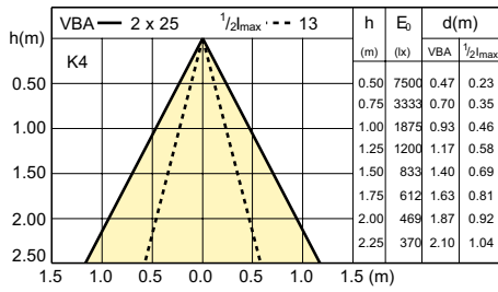
LDBE_HALUPAB_50W_25D-Beam diagram
