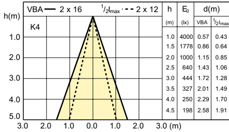
LD BE_HML111_30W_24D-Beam diagram
