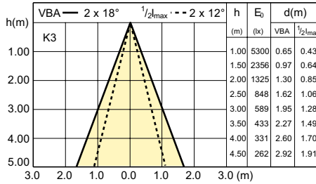
LD BE_HML111_45W_24D-Beam diagram
