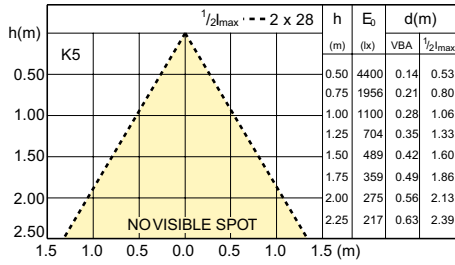
LDBE_HDICHRO_50W_60D-Beam diagram
