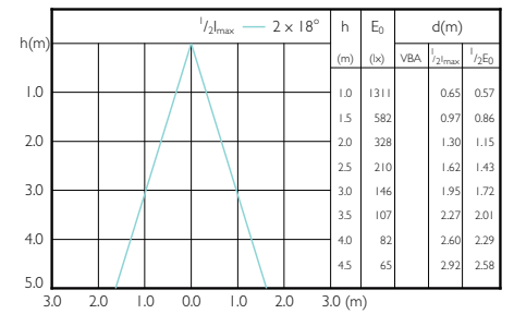
MASTER LEDspotMV 80W GU10 830 36D
