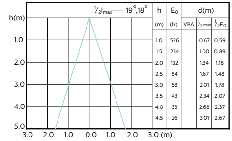
MASTER LEDspotMV 35W GU10 36D 260lm
