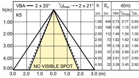
SDBE_LEDspotM_0088-Beam diagram
