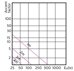
MASTER LEDspotMV 35W GU10 36D 260lm
