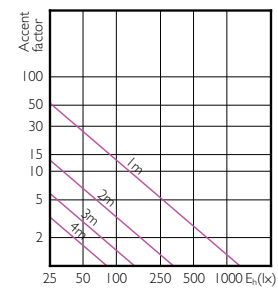
MASTER LEDspotMV 80W GU10 830 36D
