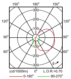
IFPS_TMS022 1xTL-D58W HFS +GMS022 R-A-Polar Normal (separate)
