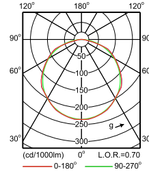
IFPS_TMS022 2xTL-D58W HFS +GMS022 R-Polar Normal (separate)
