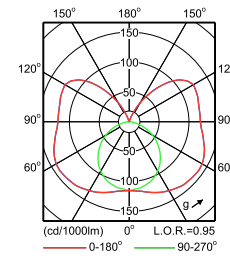
IFPS_TMS022 1xTL-D58W HFS-Polar Normal (separate)
