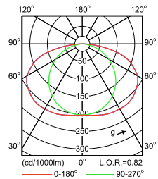
IFPS_TMS022 1xTL-D18W HFS +GMS022 R-Polar Normal (separate)
