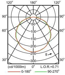
IFPS_TMS022 2xTL-D36W HFS +GMS022 R-Polar Normal (separate)
