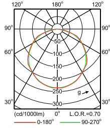
IFPS_TMS022 2xTL-D58W +GMS022 R-Polar Normal (separate)
