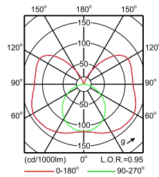
IFPS_TMS022 1xTL-D36W HFS-Polar Normal (separate)
