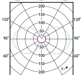
(cd/1000lm) 0-180° 90-270°
