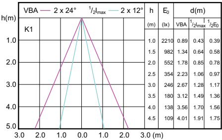
MAS LED ExpertColor 7.2-50W MR16 GU5.3 940 24D
