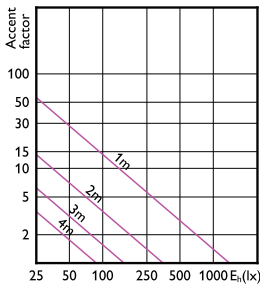
Accent Diagram - MASTER LED 6.5-50W 940 MR16 36D Dim CN
