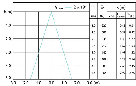
Beam diagram - MASTER LED 6.5-50W 927 MR16 36D Dim CN
