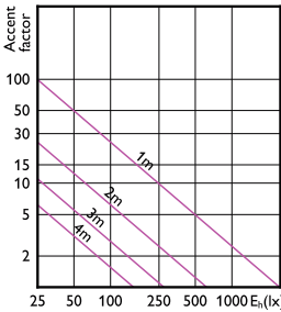
Accent Diagram - MASTER LED 6.5-50W 927 MR16 24D Dim CN
