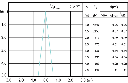
Beam diagram - MASTER LED 6.5-50W 940 MR16 10D Dim CN
