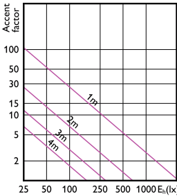
Accent Diagram - MASTER LED 6.5-50W 940 MR16 24D CN
