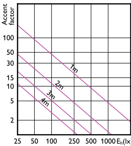
Accent Diagram - MASTER LED 6.5-50W 927 MR16 10D Dim CN
