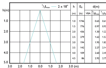
Beam diagram - MASTER LED 7.5-50W+ 830 MR16 36D Dim CN
