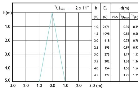
Beam diagram - MASTER LED 6.5-50W 927 MR16 24D Dim CN
