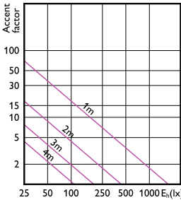
Accent Diagram - MASTER LED 7.5-50W+ 830 MR16 36D Dim CN
