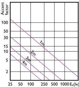
Accent Diagram - MASTER LED 7.5-50W+ 830 MR16 24D Dim CN
