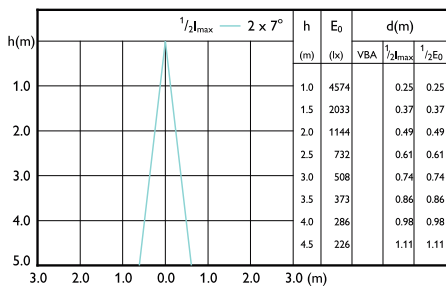
Beam diagram - MASTER LED 6.5-50W 927 MR16 10D Dim CN
