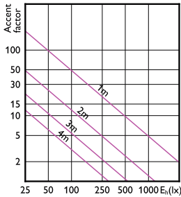
Accent Diagram - MASTER LED 6.5-50W 940 MR16 10D Dim CN
