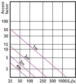
Accent Diagram - MASTER LED 6.5-50W 927 MR16 36D CN
