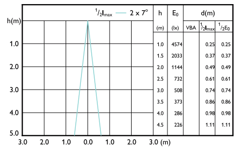
Beam diagram - MASTER LED 6.5-50W 930 MR16 10D Dim CN
