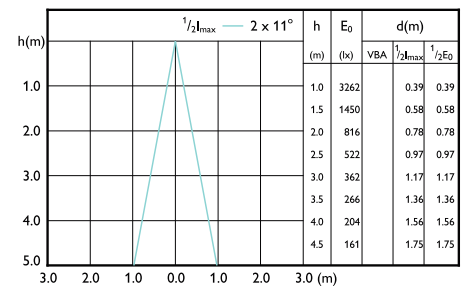
Beam diagram - MASTER LED 7.5-50W+ 830 MR16 24D Dim CN
