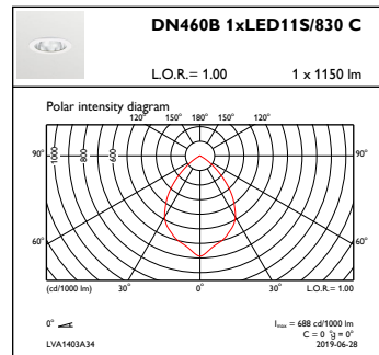
OFPC1_DN460B1xLED11S830C
