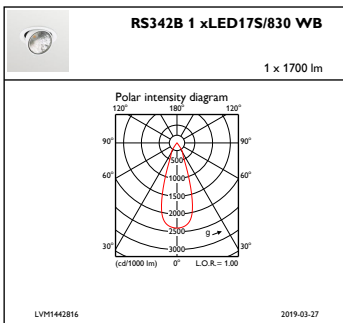
IFPC1_RS342B1xLED17S830WB
