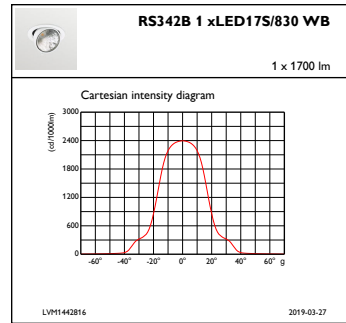
IFCC1_RS342B1xLED17S830WB
