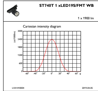
IFCC1_ST740T1xLED19SFMTWB
