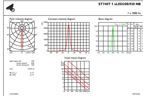
IFAS1_ST740T1xLED20S930NB
