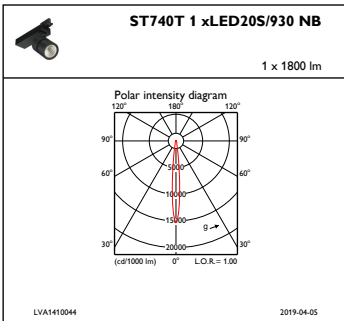
IFPC1_ST740T1xLED20S930NB
