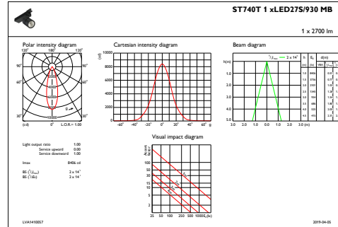
IFAS1_ST740T1xLED27S930MB
