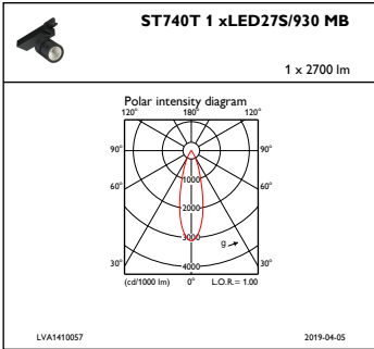
IFPC1_ST740T1xLED27S930MB
