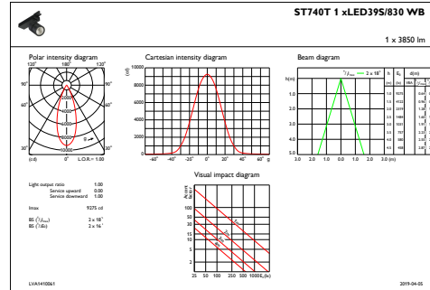
IFAS1_ST740T1xLED39S830WB
