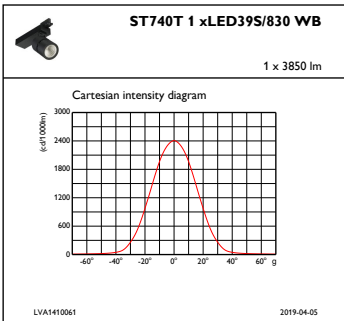
IFCC1_ST740T1xLED39S830WB
