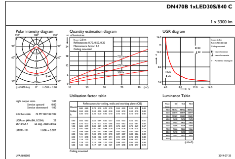
IFGU1_DN470B1xLED30S840C
