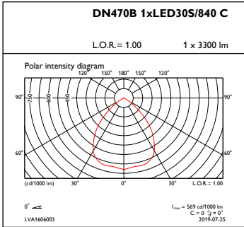
OFPC1_DN470B1xLED30S840C
