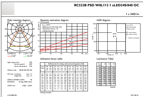
IFGU1_RC532BPSDW8L1131xLED34S840OC
