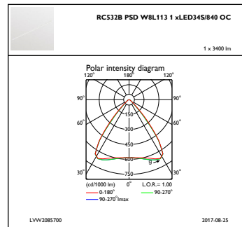
IFPC1_RC532BPSDW8L1131xLED34S840OC
