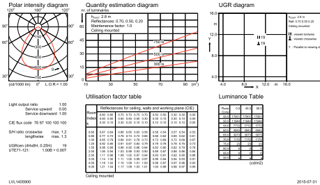
DN570B PSE-E 1xLED12S/840 C
