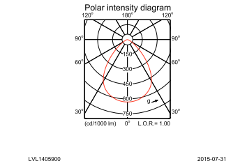
DN570B PSE-E 1xLED12S/840 C
