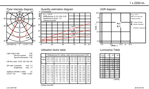
DN570B PSED-E 1xLED20S/830 F
