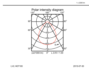
DN570B PSED-E 1xLED20S/830 F
