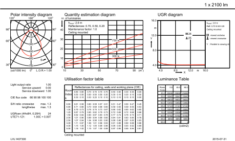
DN570B PSE-E 1xLED20S/830 WR
