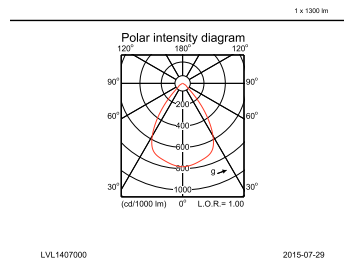
DN571B PSE-E 1xLED12S/830 F
