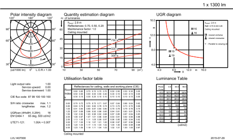
DN571B PSE-E 1xLED12S/830 F
