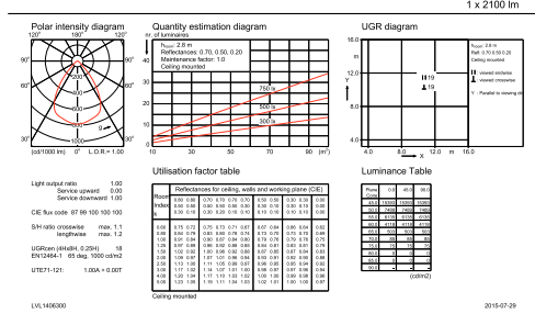
DN571B PSE-E 1xLED20S/840 C
