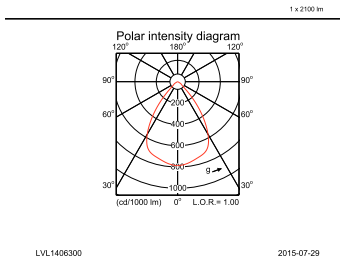
DN571B PSE-E 1xLED20S/840 C
