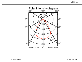
DN571B PSE-E 1xLED20S/840 F
