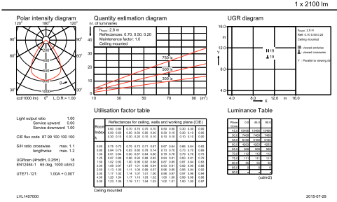
DN571B PSE-E 1xLED20S/840 F
