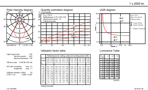
DN571B PSED-E 1xLED20S/830 WR
