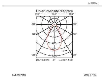
DN571B PSED-E 1xLED20S/830 WR
