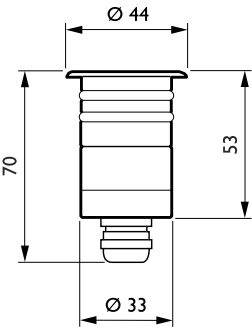
AmphiLux BBD/BVD400
