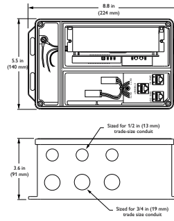
Power/data supply units ZCX400
