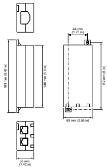
Power/data supply units ZCX400
