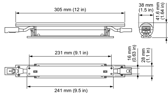
BCX416 10xLED-HB-3000 100-277V MB
