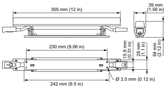
LS515X LED5/3000 100–277V MB WH
