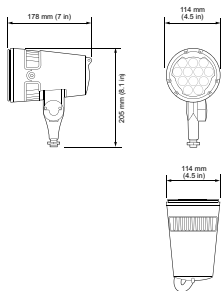
BCP463 12xLED-HB-4000 100-277V HMA BK CE
