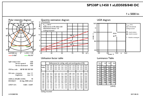
IFGU1_SP530PL14501xLED50S840OC
