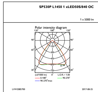
IFPC1_SP530PL14501xLED50S840OC
