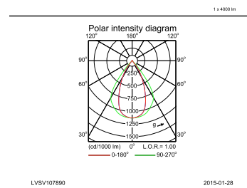
IFPC1_4MX400 G3 491 1xLED40S830 PSD NB.EPS
