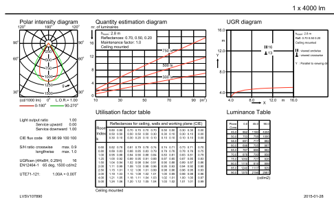
IFGU1_4MX400 G3 491 1xLED40S830 PSD NB.EPS
