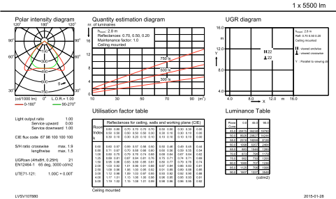
IFGU1_4MX400 G3 491 1xLED55S840 PSD WB.EPS
