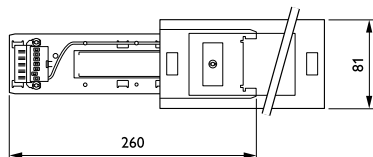
CoreLine trunking LL120X/LL121X
