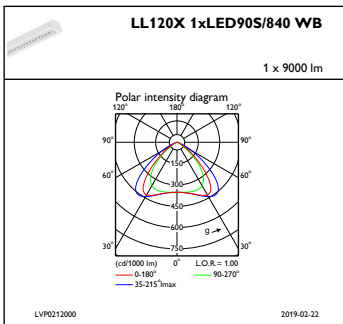
IFPC1_LL120X1xLED90S840WB
