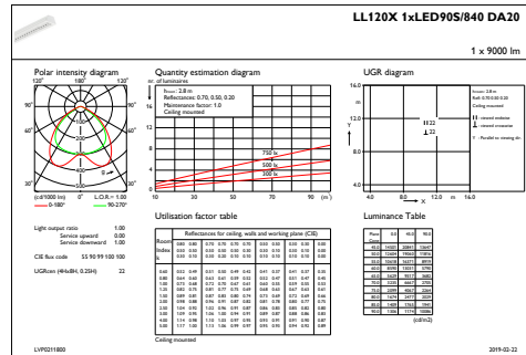
IFGU1_LL120X1xLED90S840DA20
