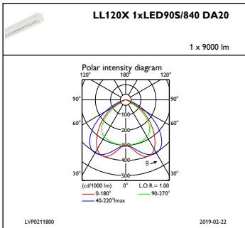
IFPC1_LL120X1xLED90S840DA20
