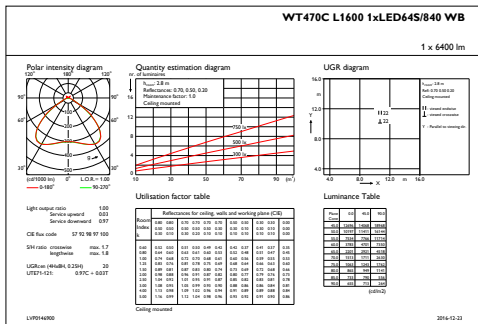
IFGU1_WT470C L1600 1xLED64S840WB
