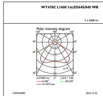
IFPC1_WT470C L1600 1xLED64S840WB
