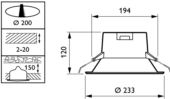
DN060B LED18S/840 PSU WH
