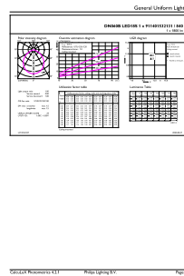
Downlight DN060B LED18S 840 PSU WH
